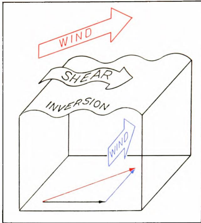
Inversion Waves
